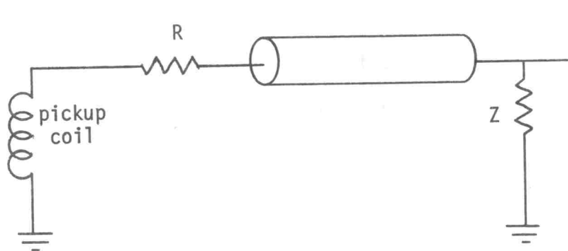
Fig. 4.4.--Pickup coil circuit.
